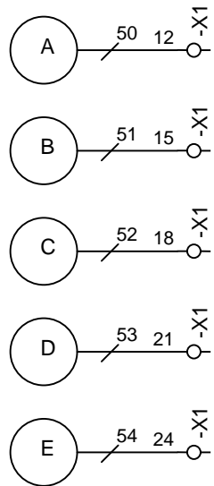
Socket Connector
